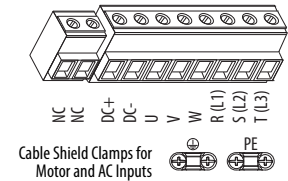
Power Terminal Block 2099-BM09-S
