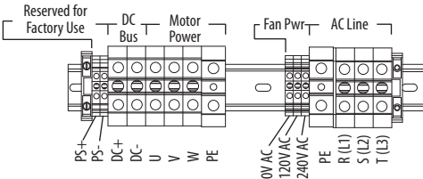
Power Terminal Block 2099-BM09-S
