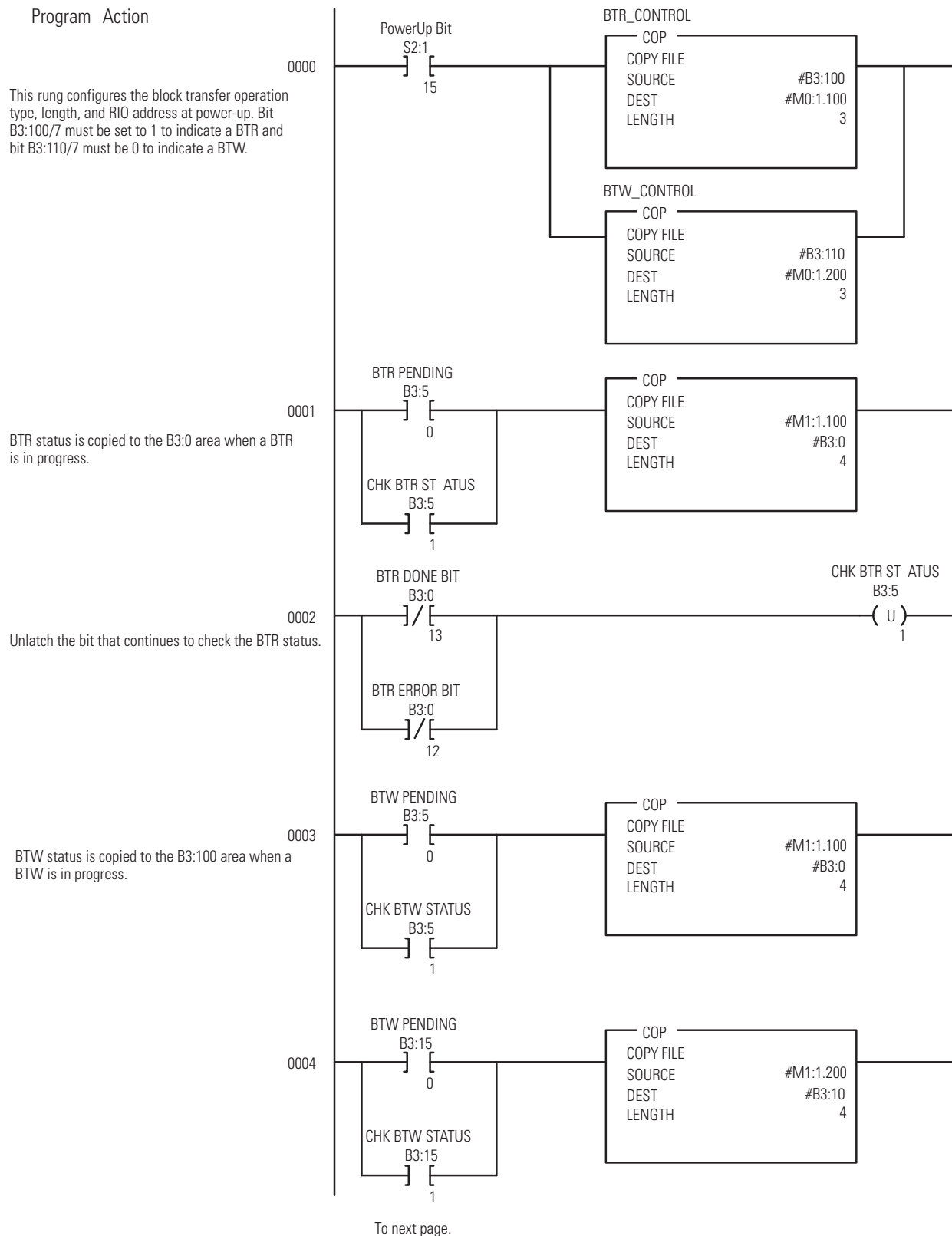
Figure 1.9 SLC Programming for the 1794-IF2XOF2I Isolated Analog Input/Output Module
