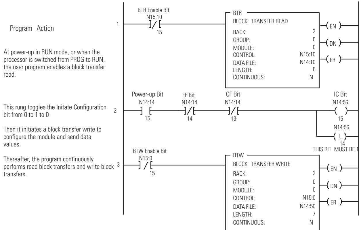
Figure 1.5 PLC-5 Family Sample Program Structure for the 1794-0F4I
