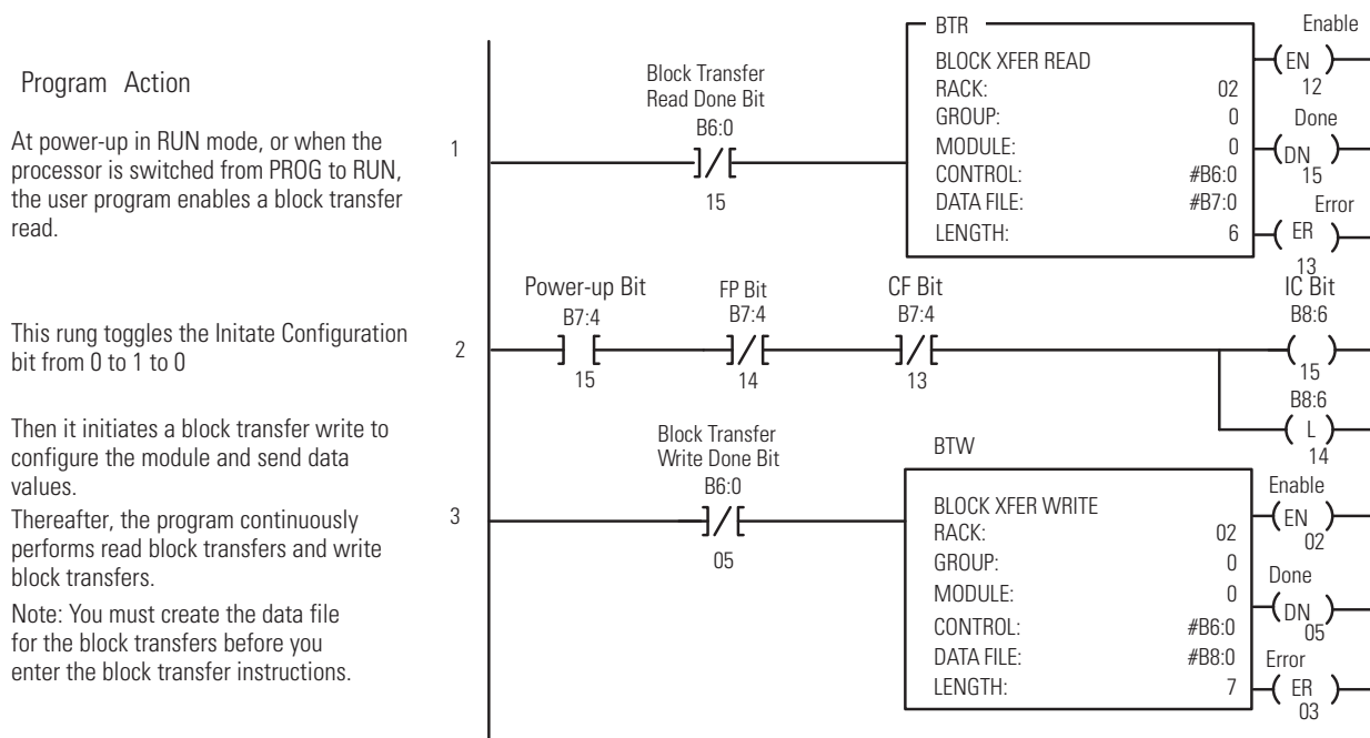
Figure 1.2 PLC-3 Family Sample Program Structure for a 1794-OF4I Module
