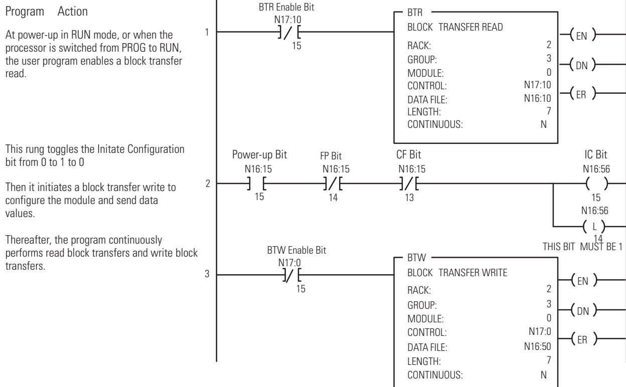
Figure 1.6 PLC-5 Family Sample Program Structure for the 1794-IF2XOF2I
