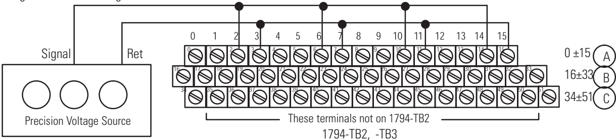
Figure 7.1 Calibration Set-Ups
