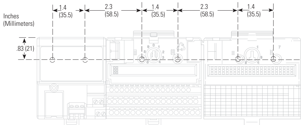
Figure 2.3 Drilling Dimensions for Panel/Wall Mounting of FLEX I/O
