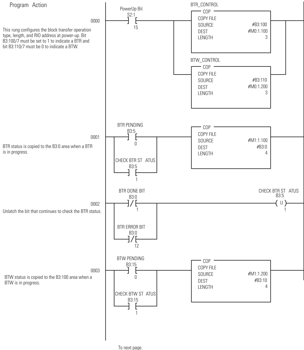
Figure 1.8 SLC Programming for the 1794-IF4I Isolated Analog Input Module
